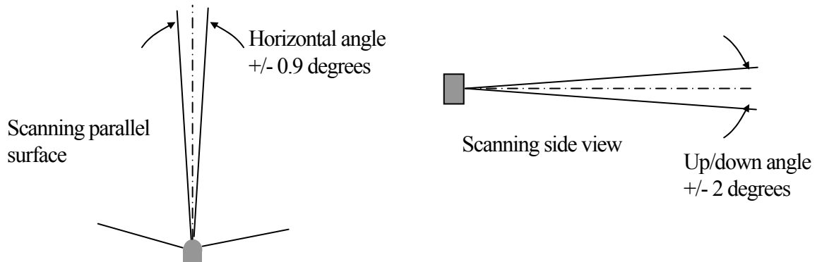
Dispersion between optical axis and mechanical axis
