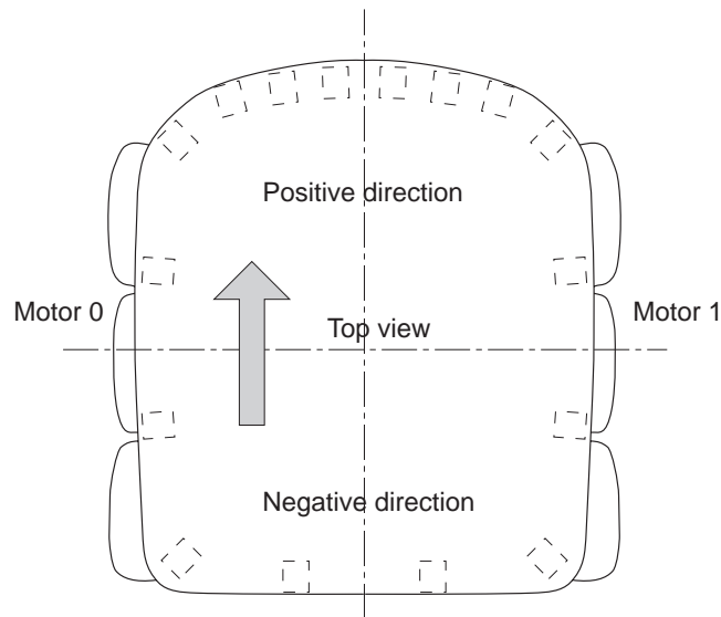
Figure 3: Motor number and direction position
