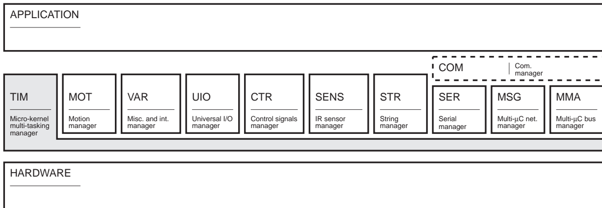
Figure 1: General topology of the BIOS
