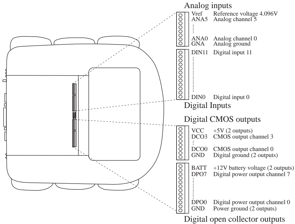
Figure 8: General I/O port definitions
